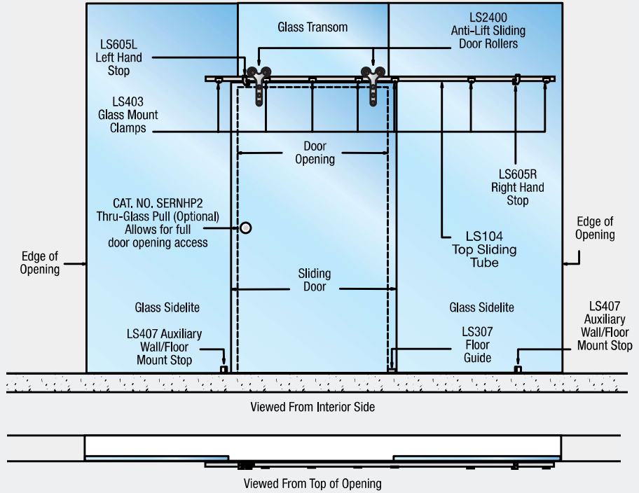
TYPICAL LSGM26 KIT SHOWN
